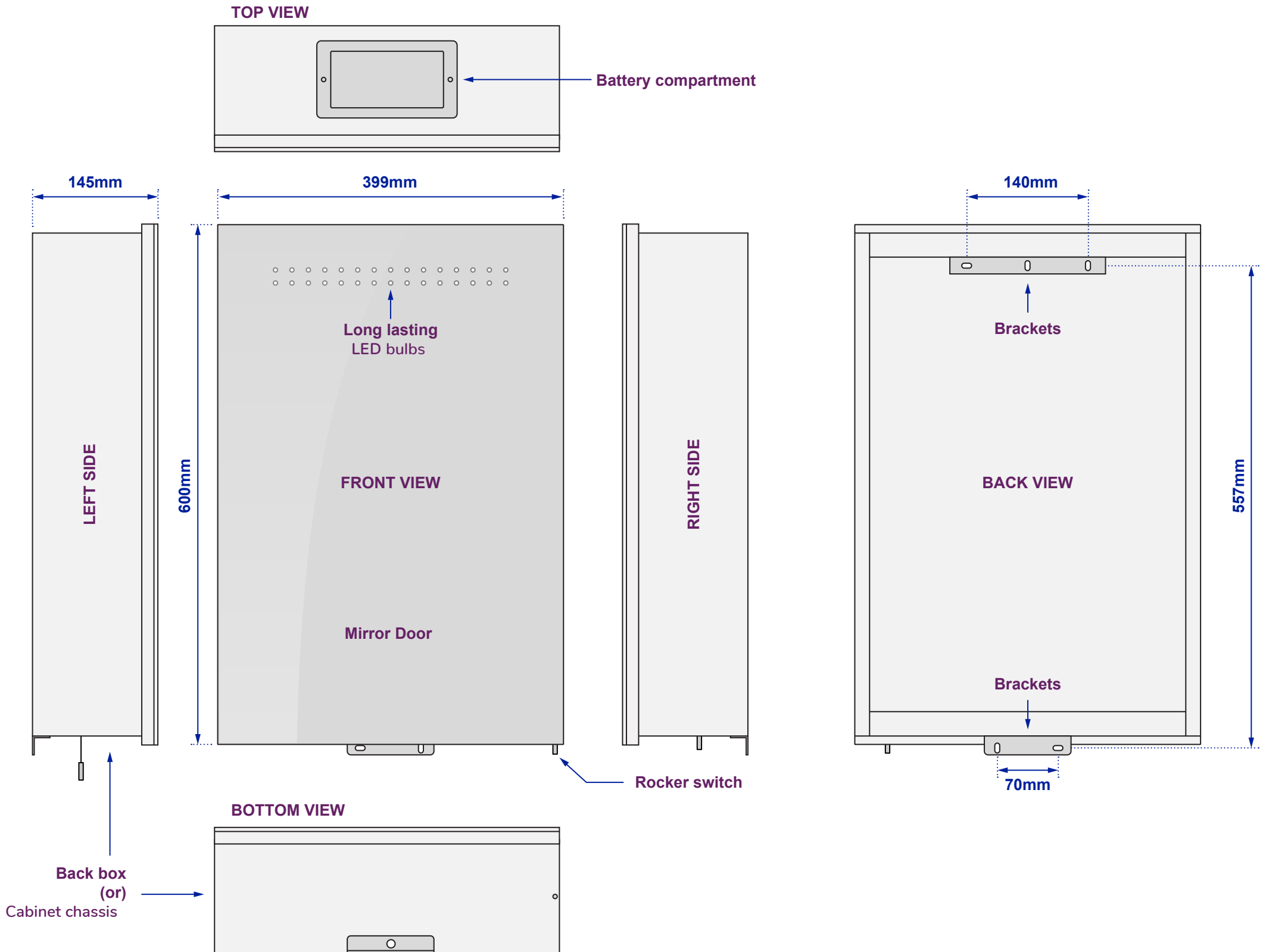
Views of complete assembly - With Mirror Door(s) / Panel(s)
