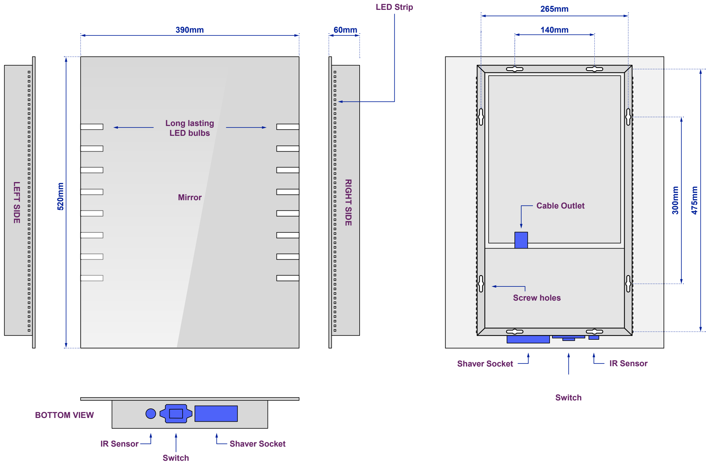
Views of complete assembly
