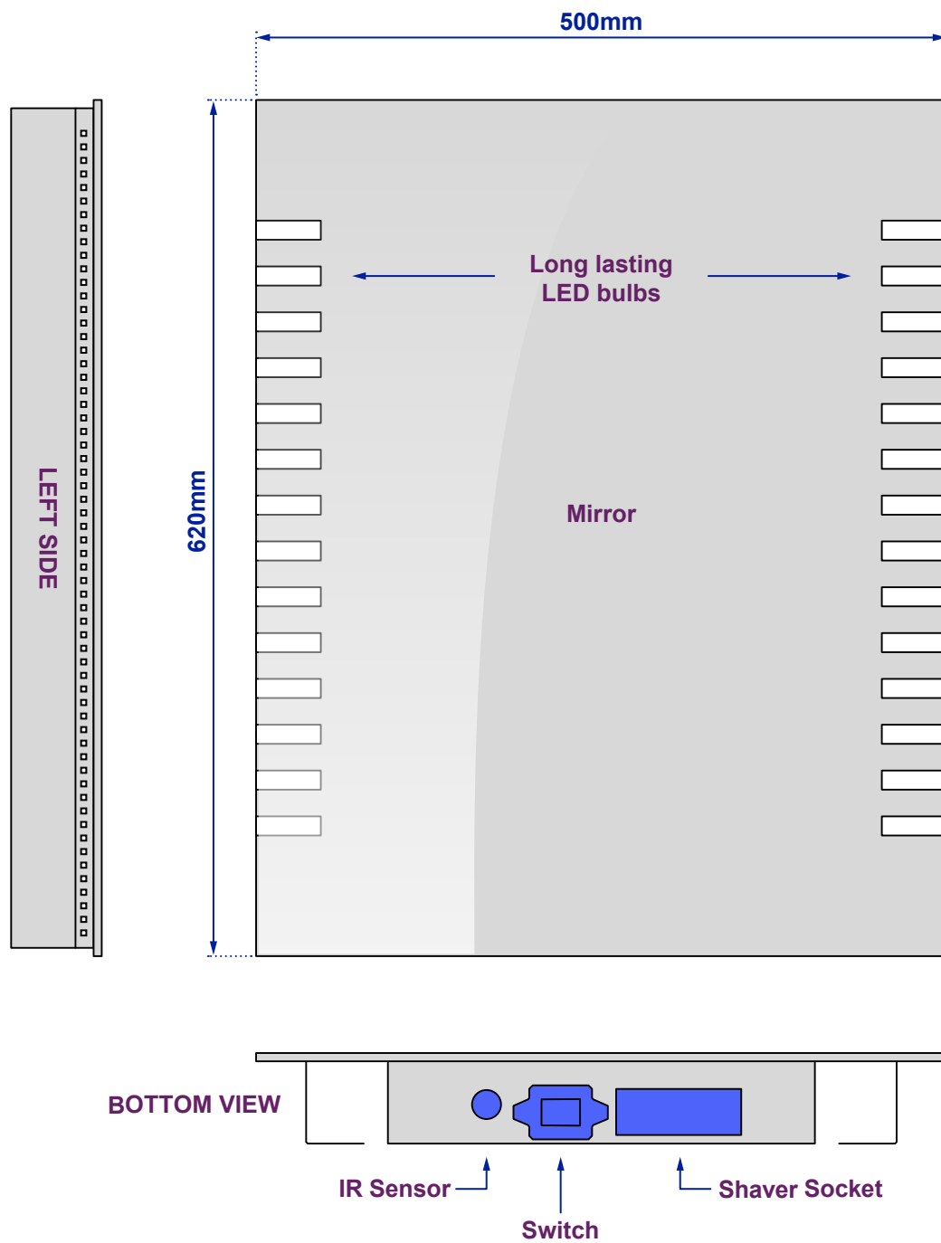
Views of complete assembly
