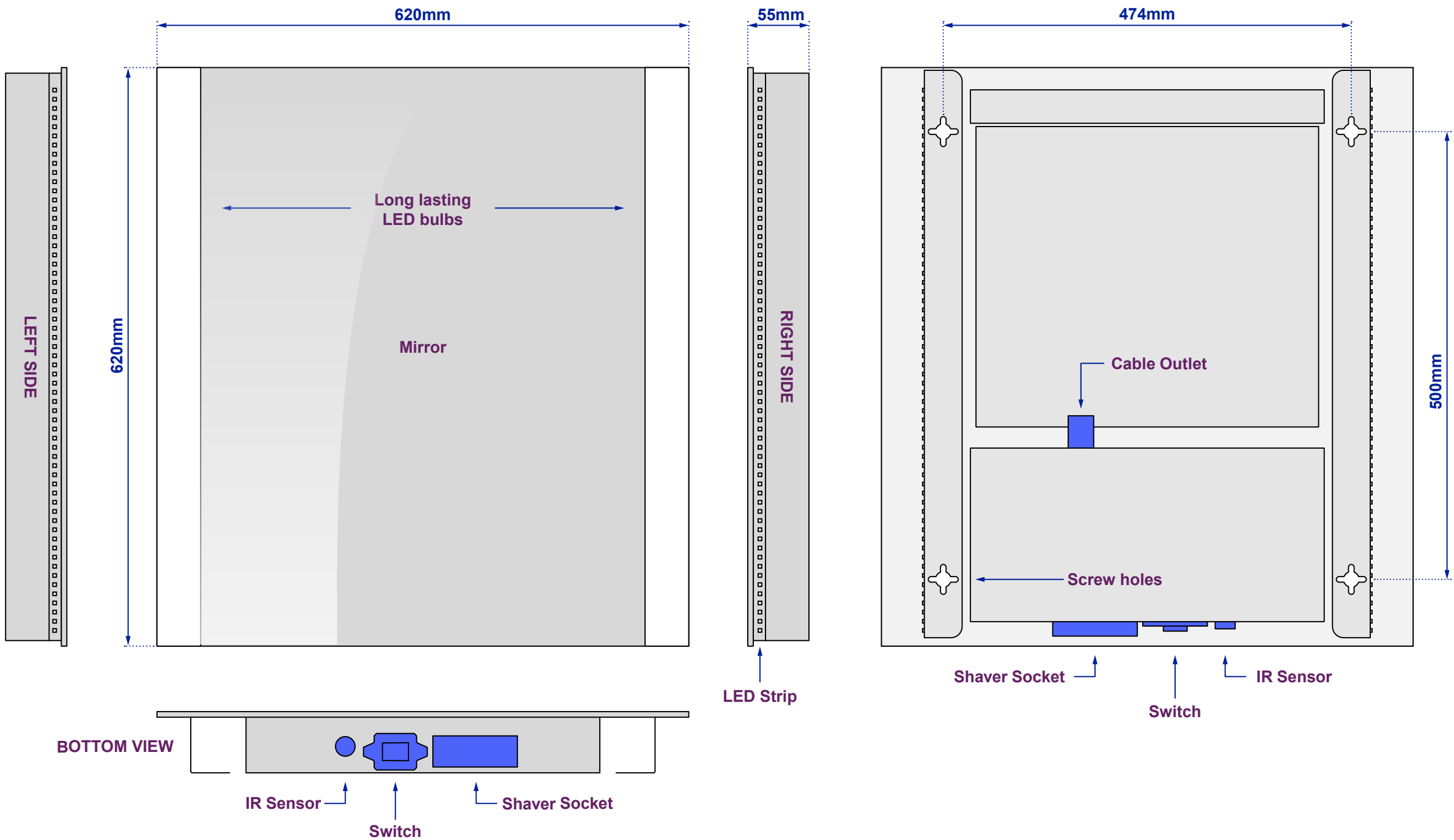
View of Back plate
