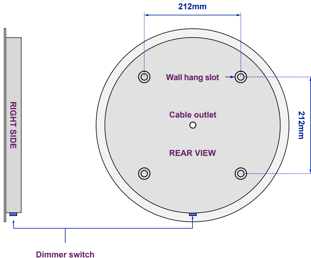
Views of Back plate - Without Mirror
