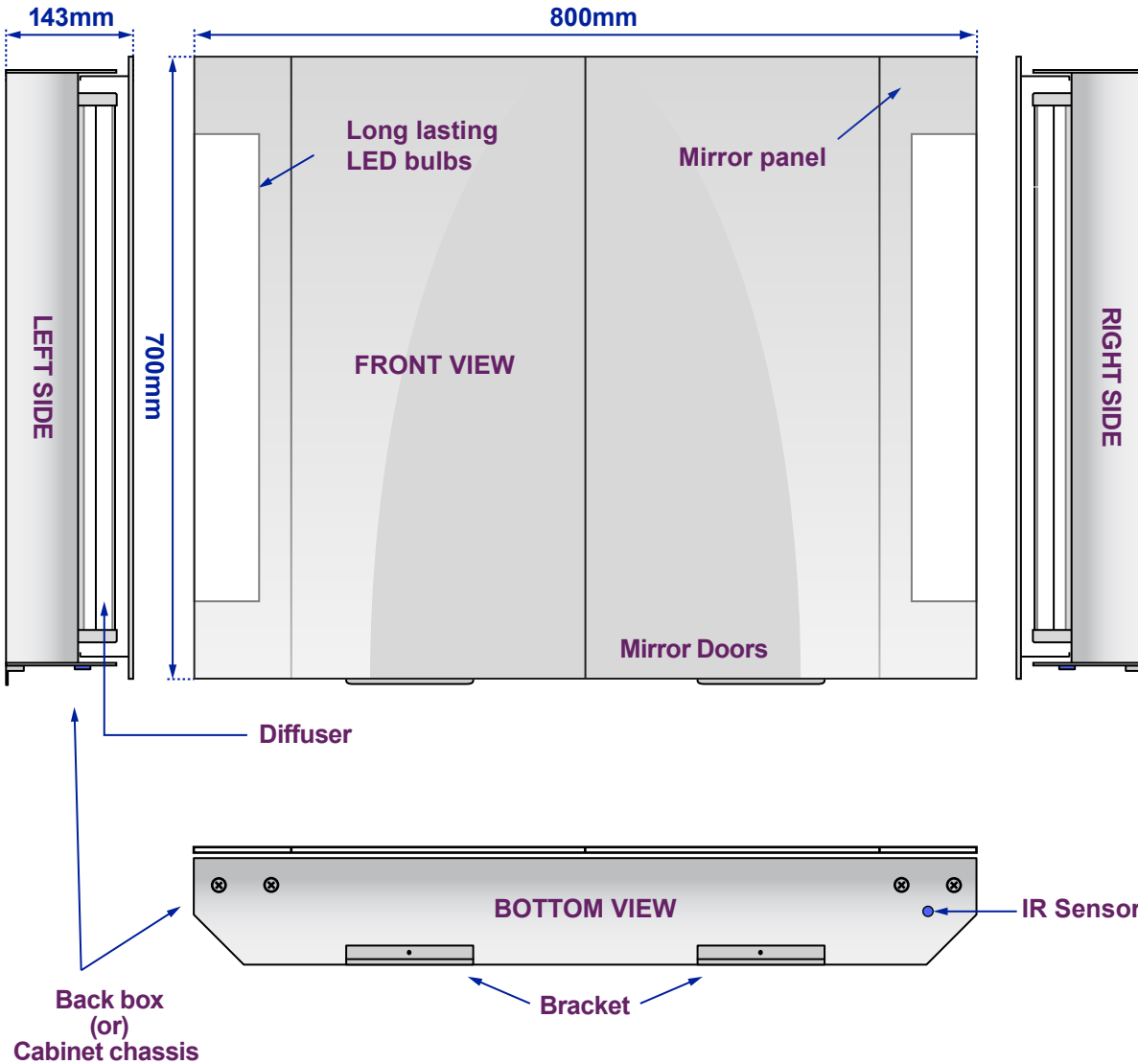
Views of complete assembly - With Mirror Door(s)/Panel(s)
