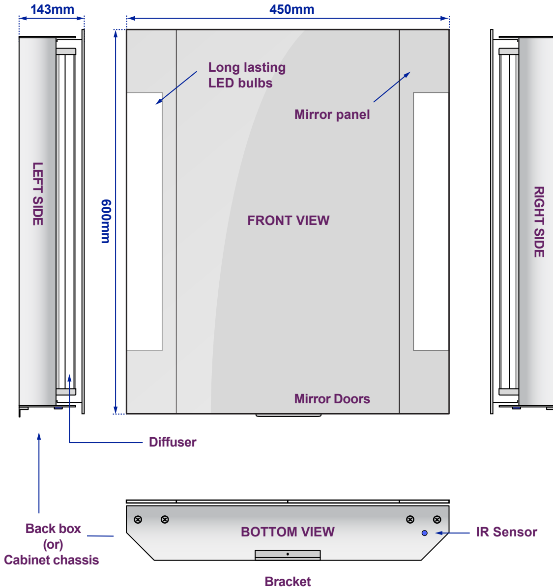
Views of complete assembly - With Mirror Door(s)/Panel(s)
