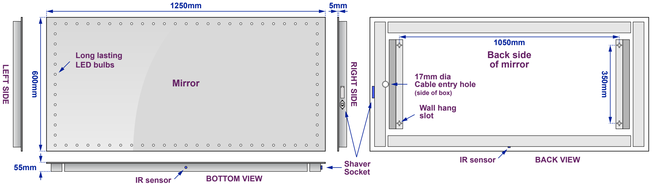
Views of complete assembly
