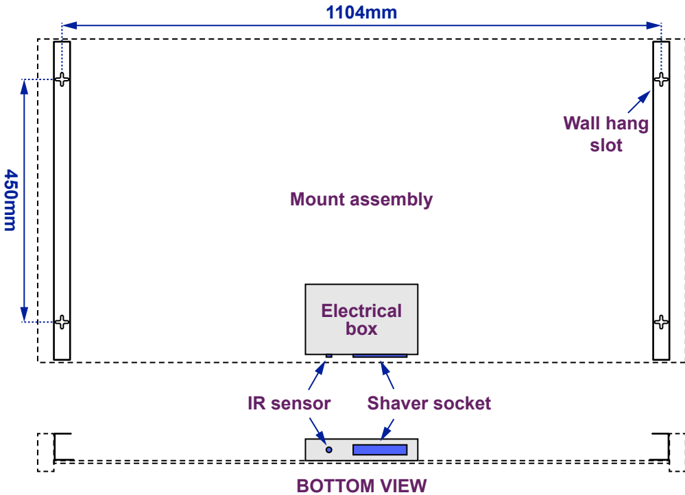
Views of Mount assembly - Without Mirror and light boxes
