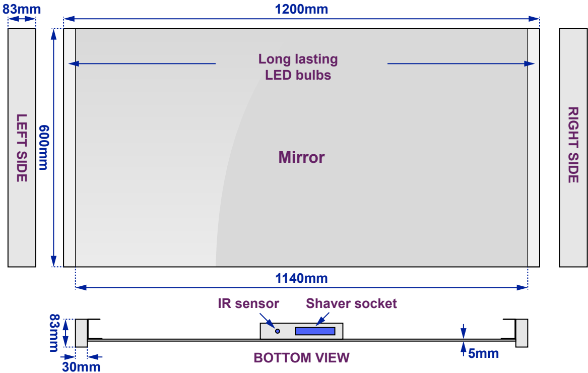
Views of complete assembly - With Mirror and light boxes
