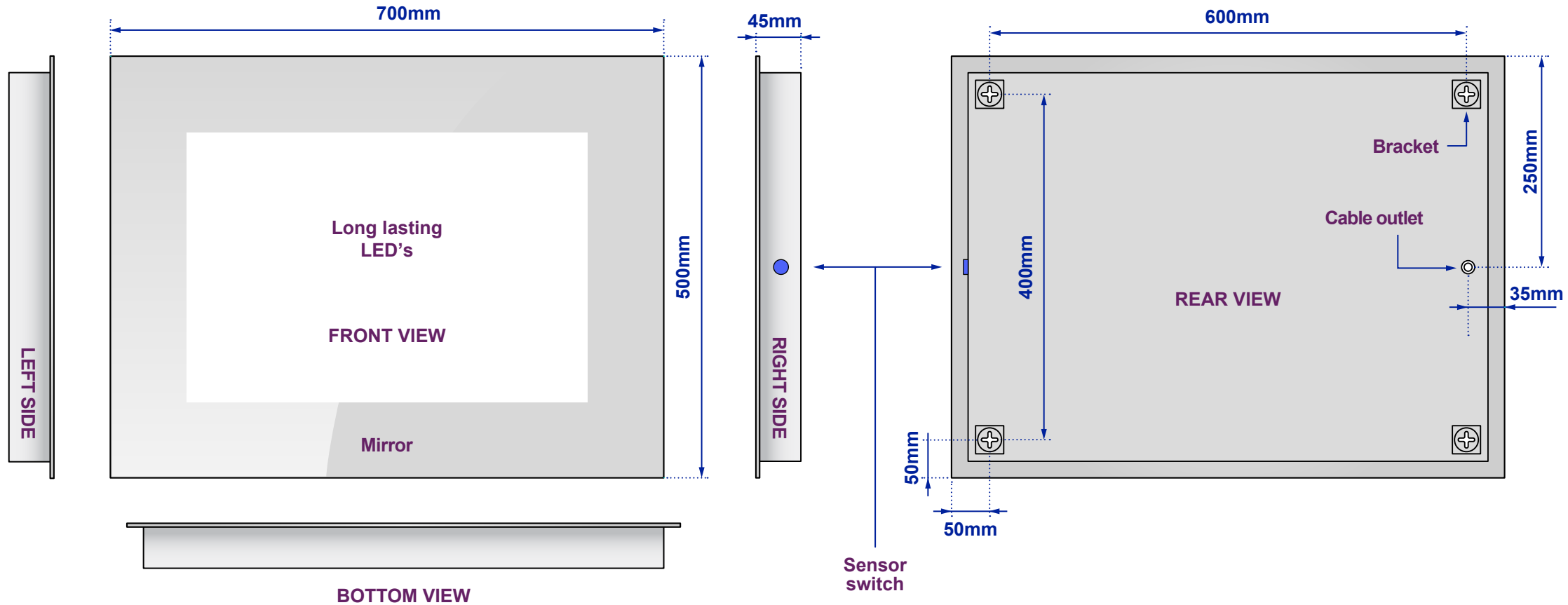
View of Back plate
