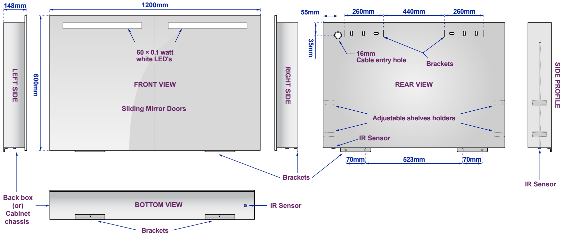
Views of complete assembly - With Mirror Door(s)/Panel(s)
