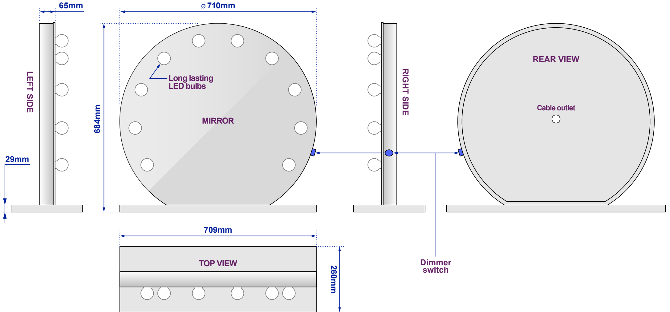
Views of completed assembly
