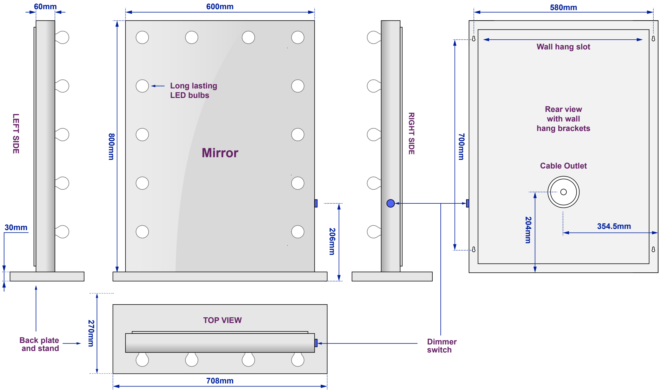
Views of completed stand assembly - with bulbs in place
