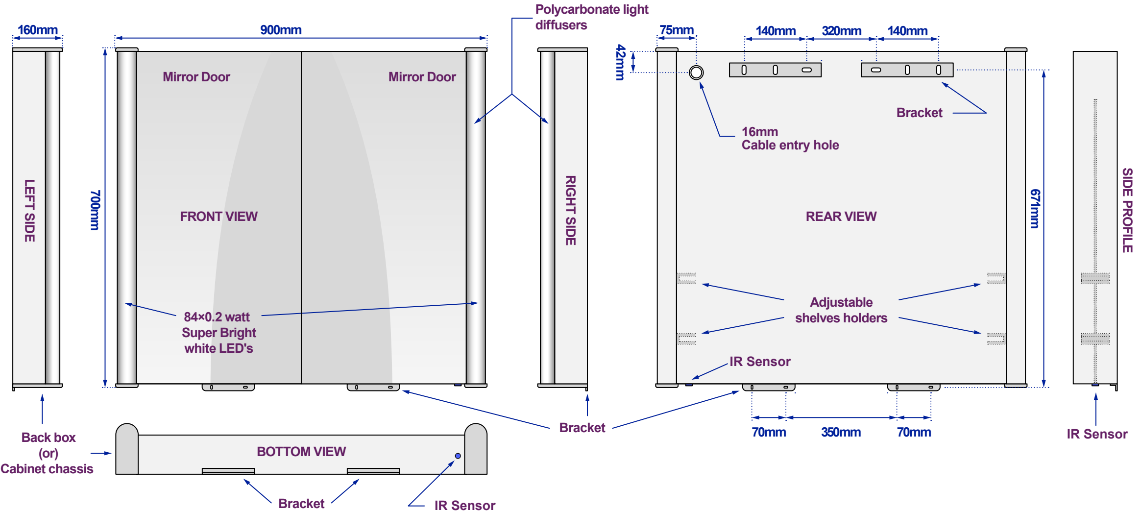
Views of complete assembly - With Mirror Door(s)
