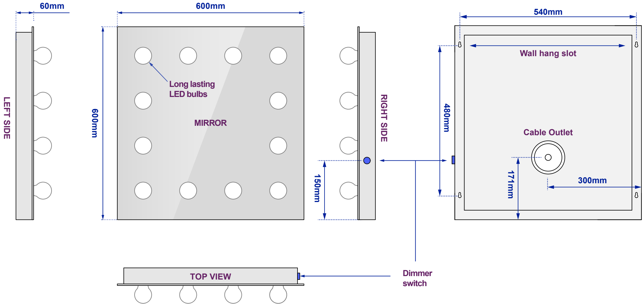
Views of completed assembly - with bulbs in place
