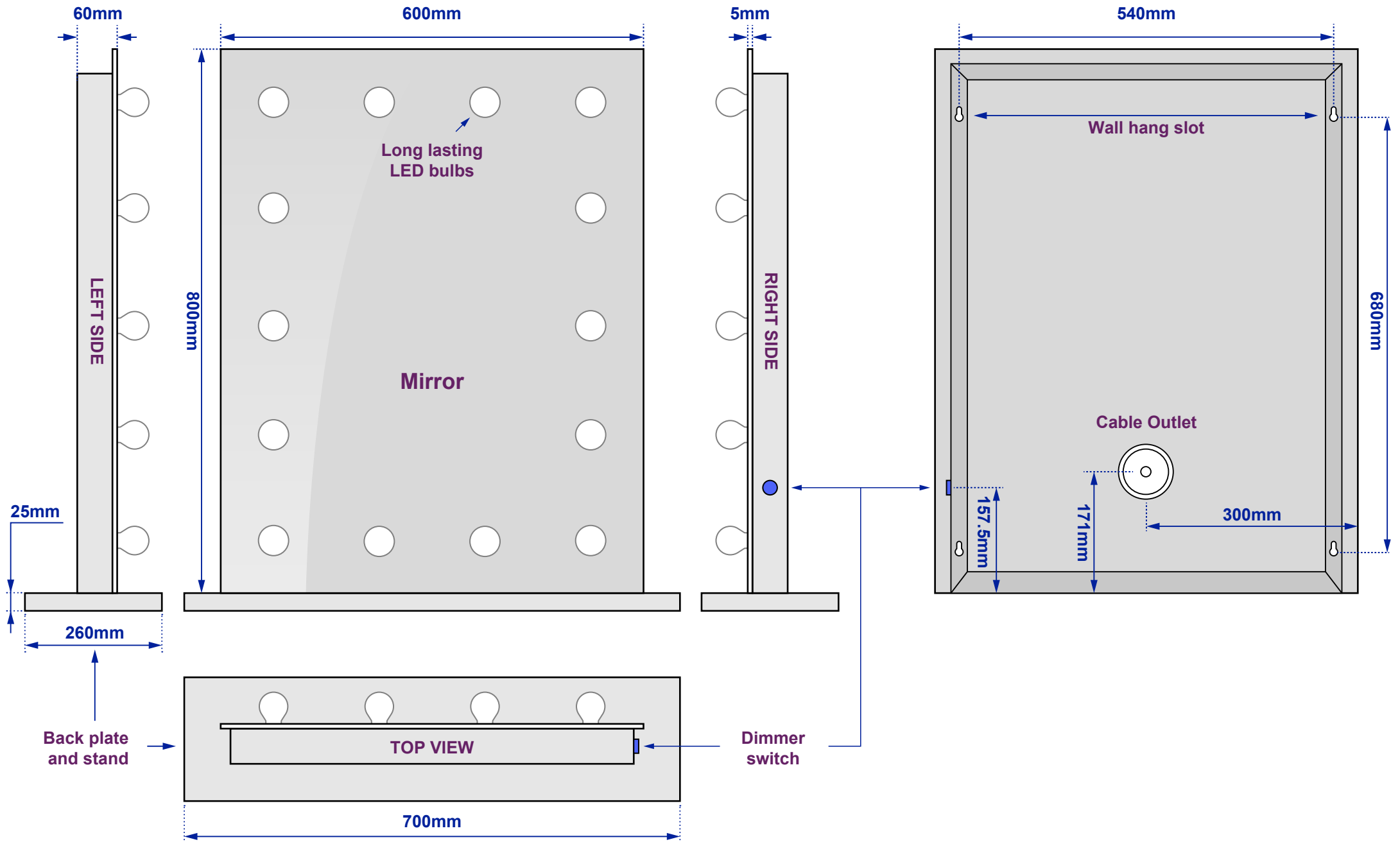
Views of complete assembly - With Mirror
