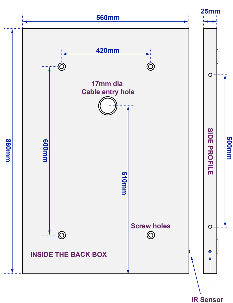
Views of Back plate - Without Mirror
