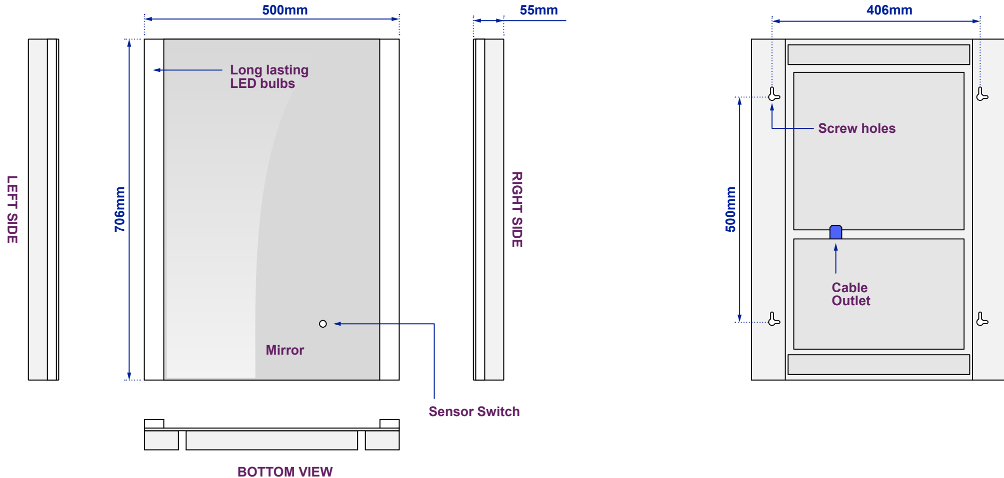
View of Back plate
