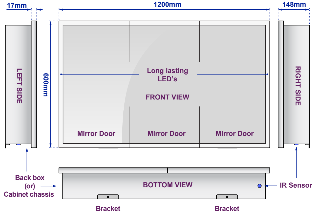
Views of complete assembly - With Mirror Door(s)/Panel(s)
