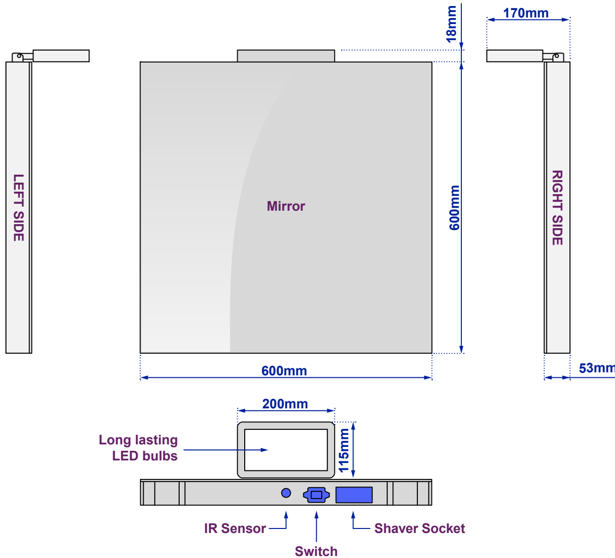
Views of complete assembly
