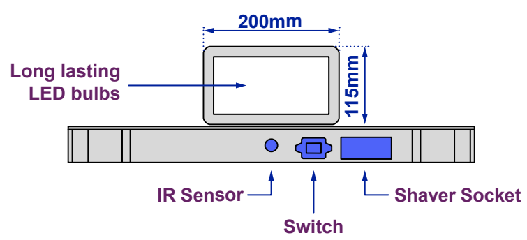
Views of complete assembly
