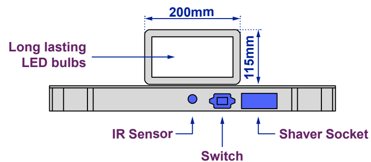
Views of complete assembly
