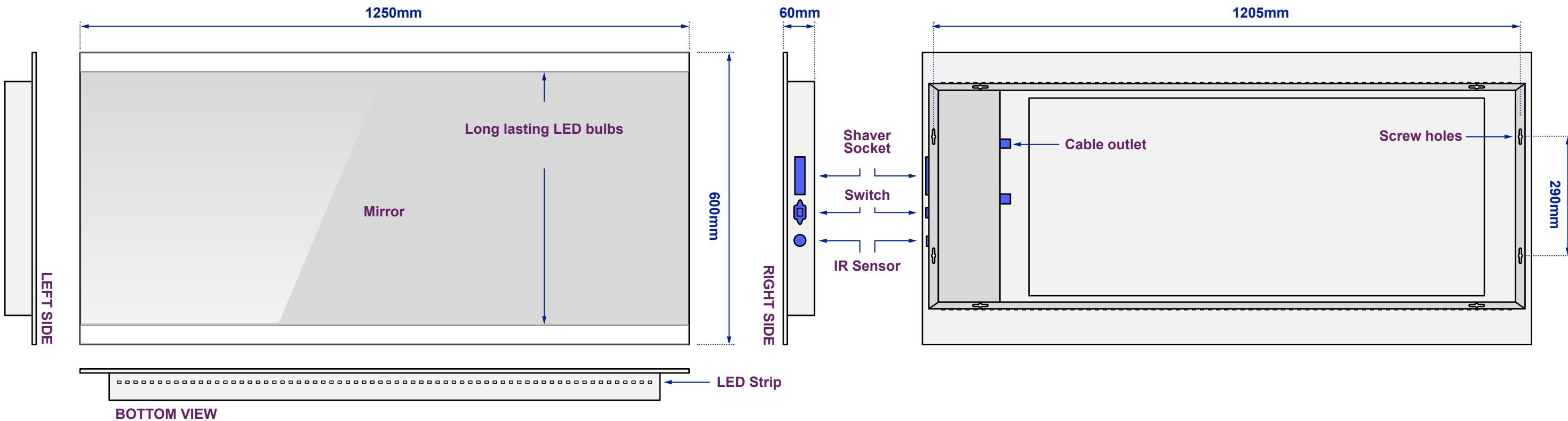
View of Back plate
