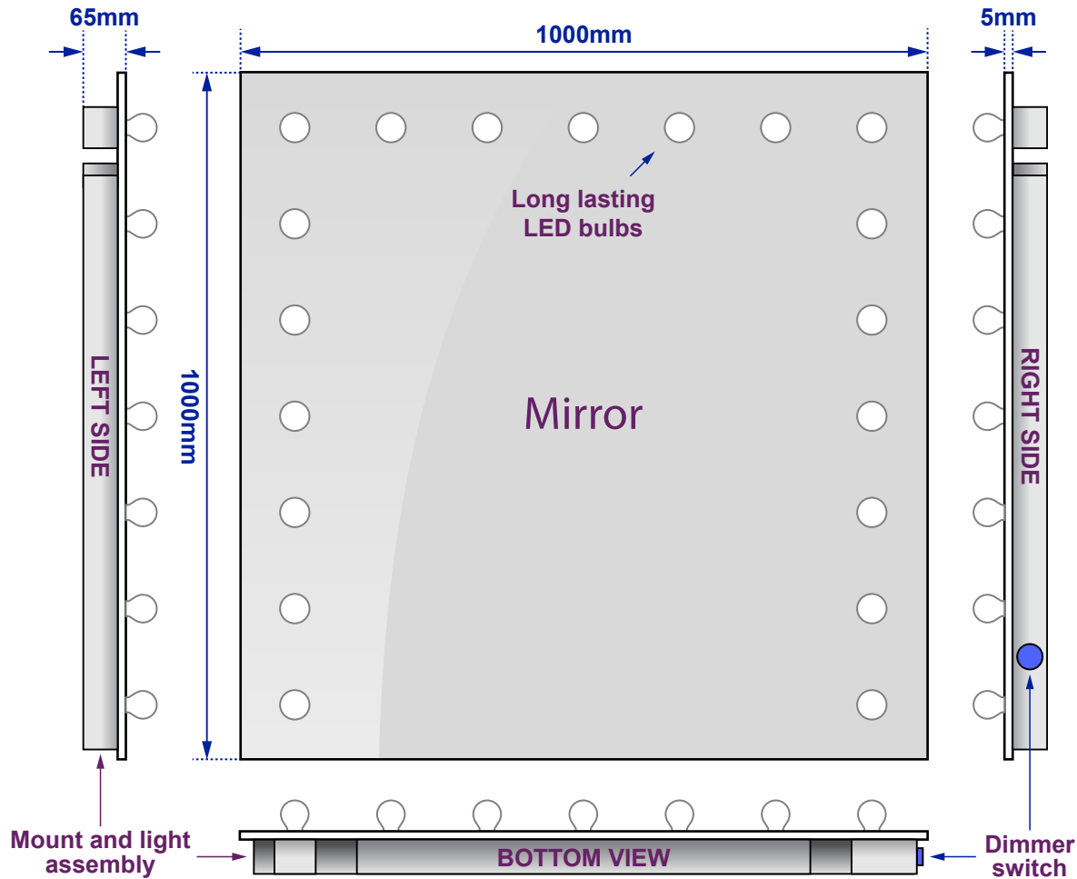
Views of complete assembly - With Mirror
