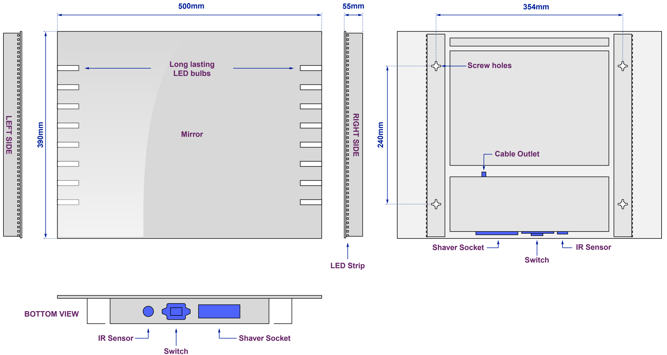
View of Back plate
